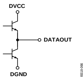
Figure 64. Logic Output
