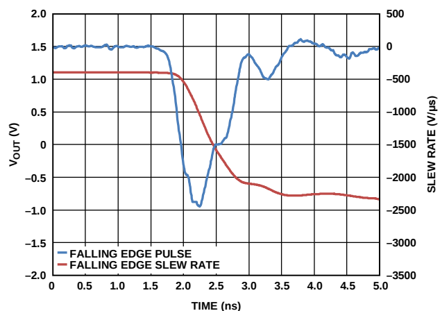
Figure 20. ADV3228 Falling Edge Slew Rate
